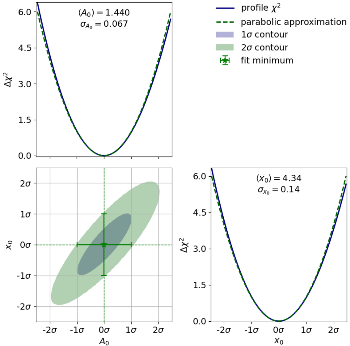
Fig. 5.4: Parameter confidence contours for the exponential fit from the model functions example. The estimators are nearly normally distributed on the scale of the uncertainty so the confidence region is close to an ellipse.
